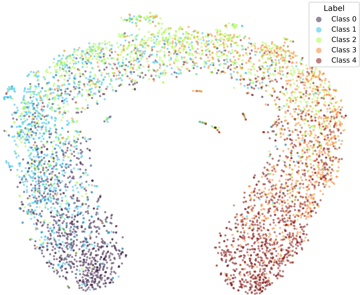
google/bert_uncased_L-2_H-128_A-2-yelp-WKL-TRIPa1-4 (val)
