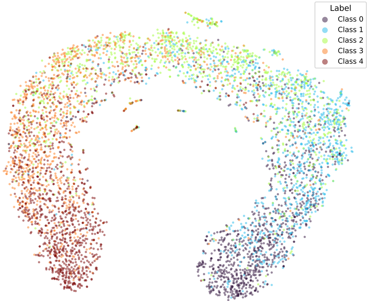
google/bert_uncased_L-2_H-128_A-2-yelp-WKL-TRIPa1-5 (val)
