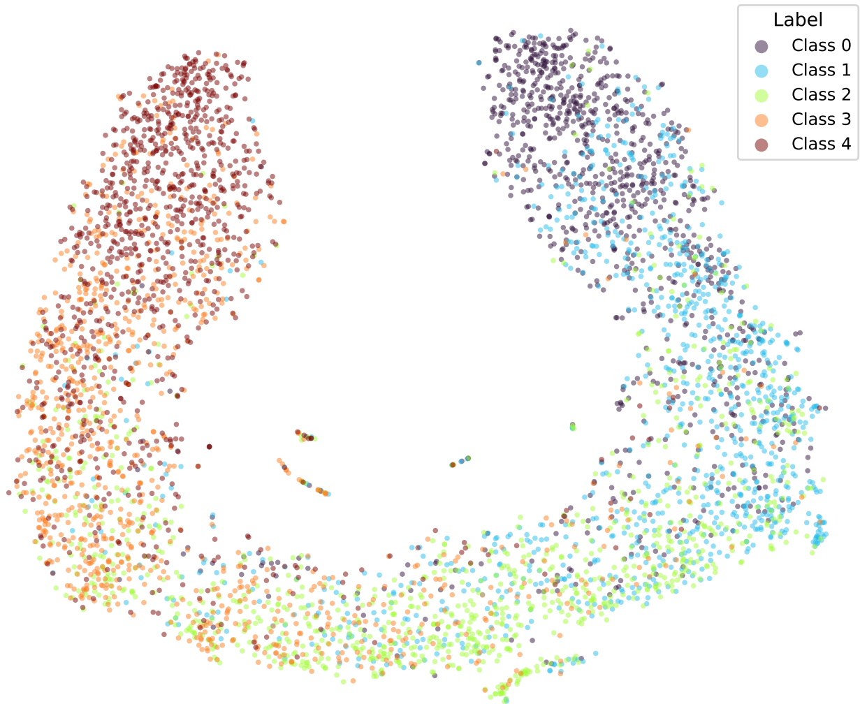
google/bert_uncased_L-2_H-128_A-2-yelp-WKL-TRIPa2-1 (val)
