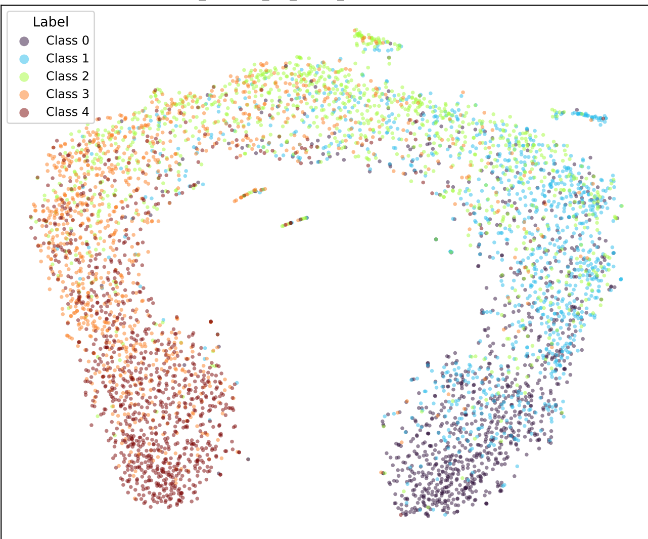
google/bert_uncased_L-2_H-128_A-2-yelp-WKL-TRIPa2-2 (val)
