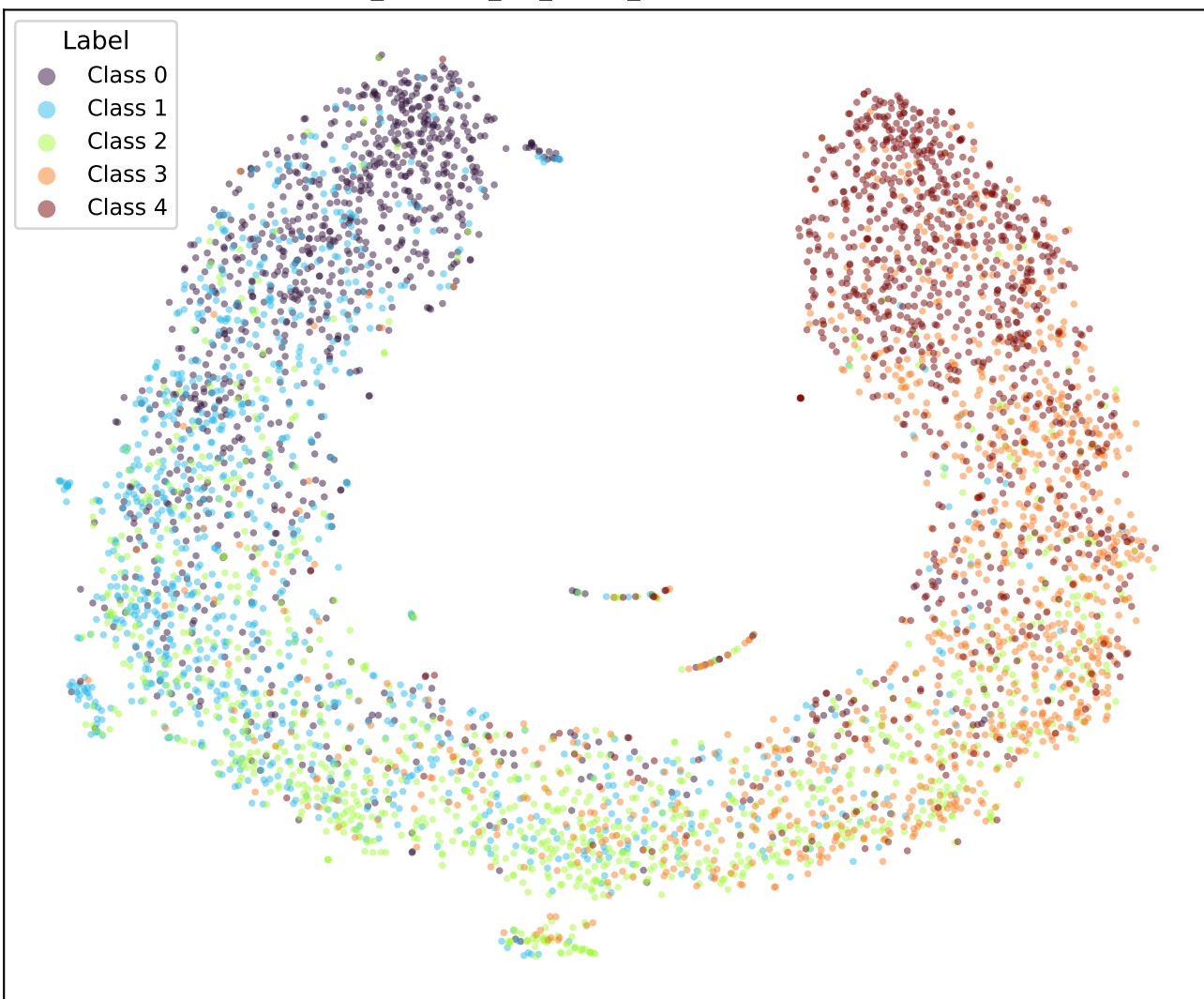
google/bert_uncased_L-2_H-128_A-2-yelp-WKL-TRIPa2-4 (val)
