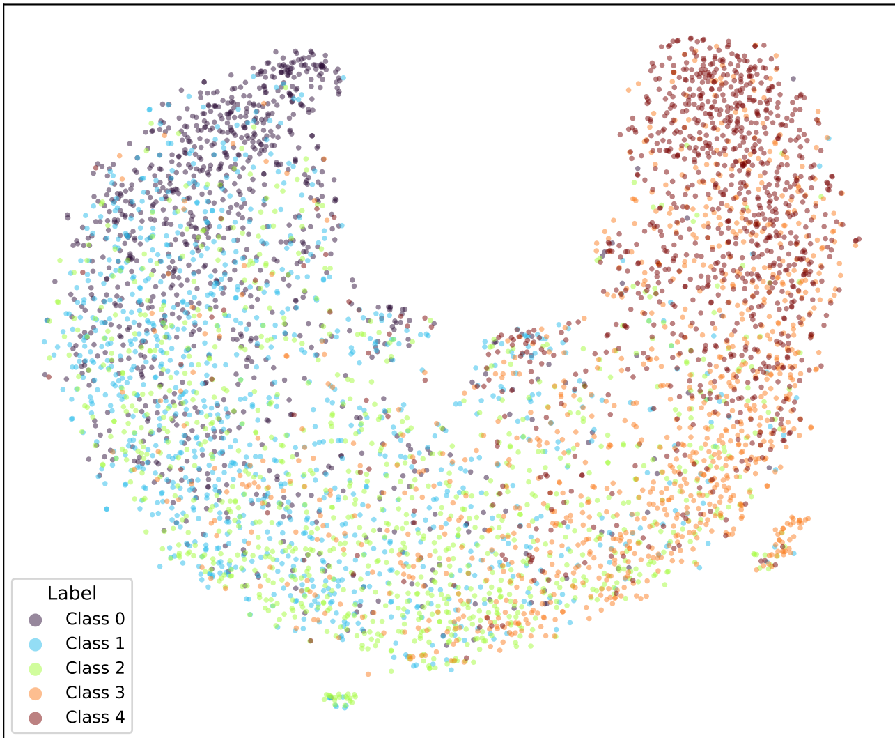
google/bert_uncased_L-2_H-128_A-2-amazon_reviews-BCE-TRIPa2-1 (val)
