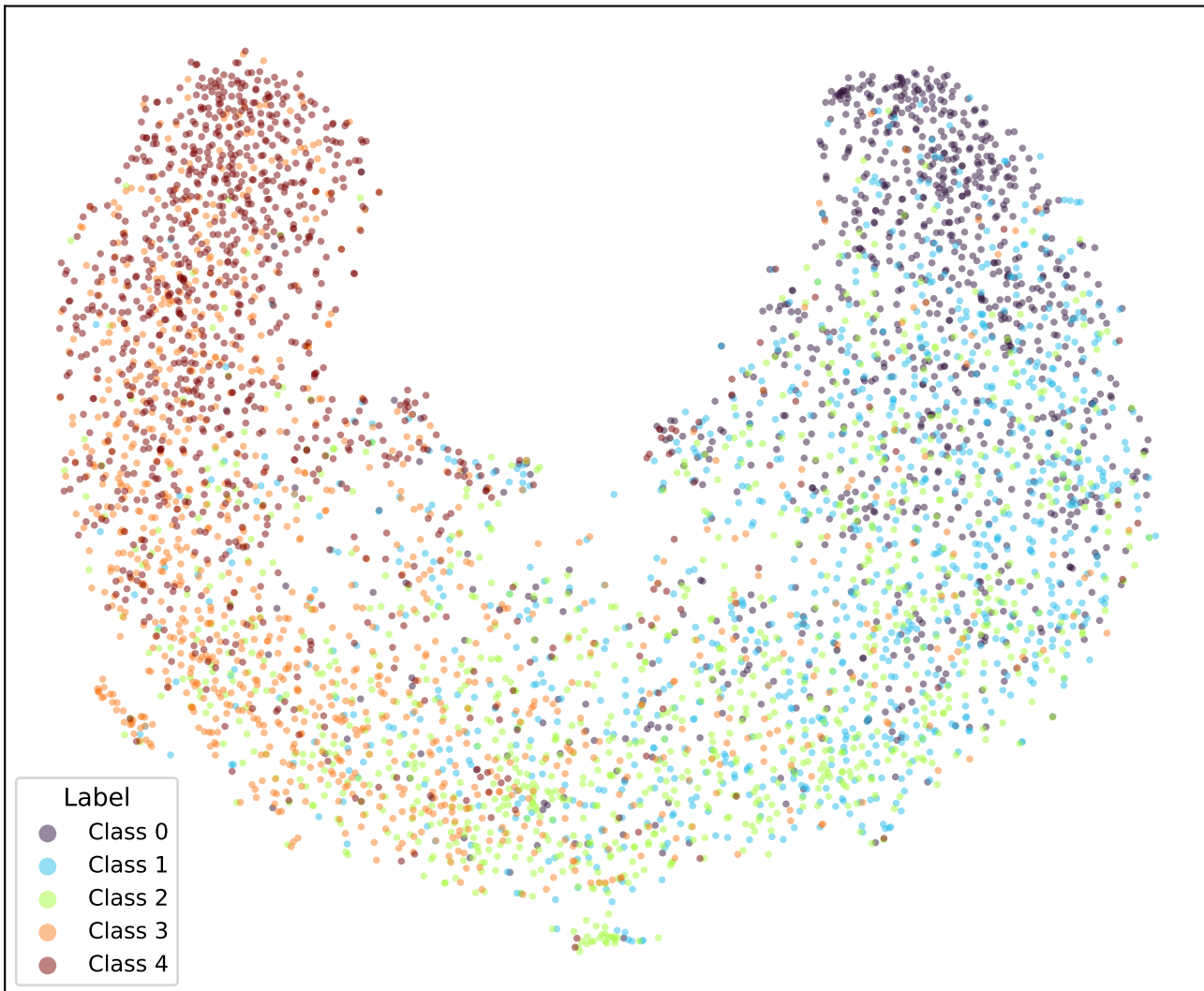
google/bert_uncased_L-2_H-128_A-2-amazon_reviews-BCE-TRIPa2-4 (val)
