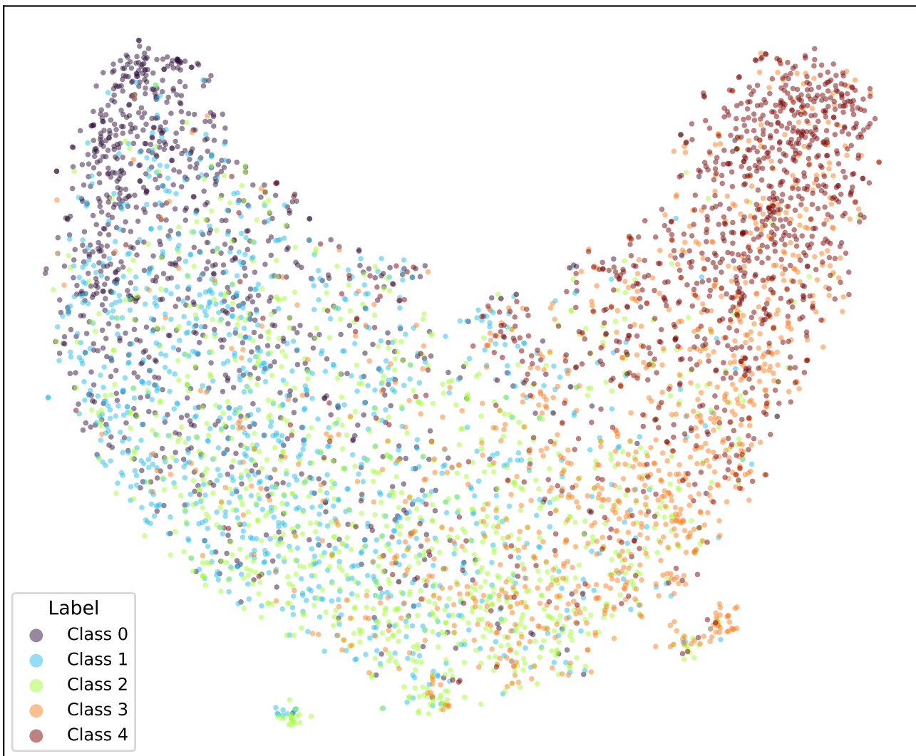
google/bert_uncased_L-2_H-128_A-2-amazon_reviews-CE-TRIPa2-2 (val)
