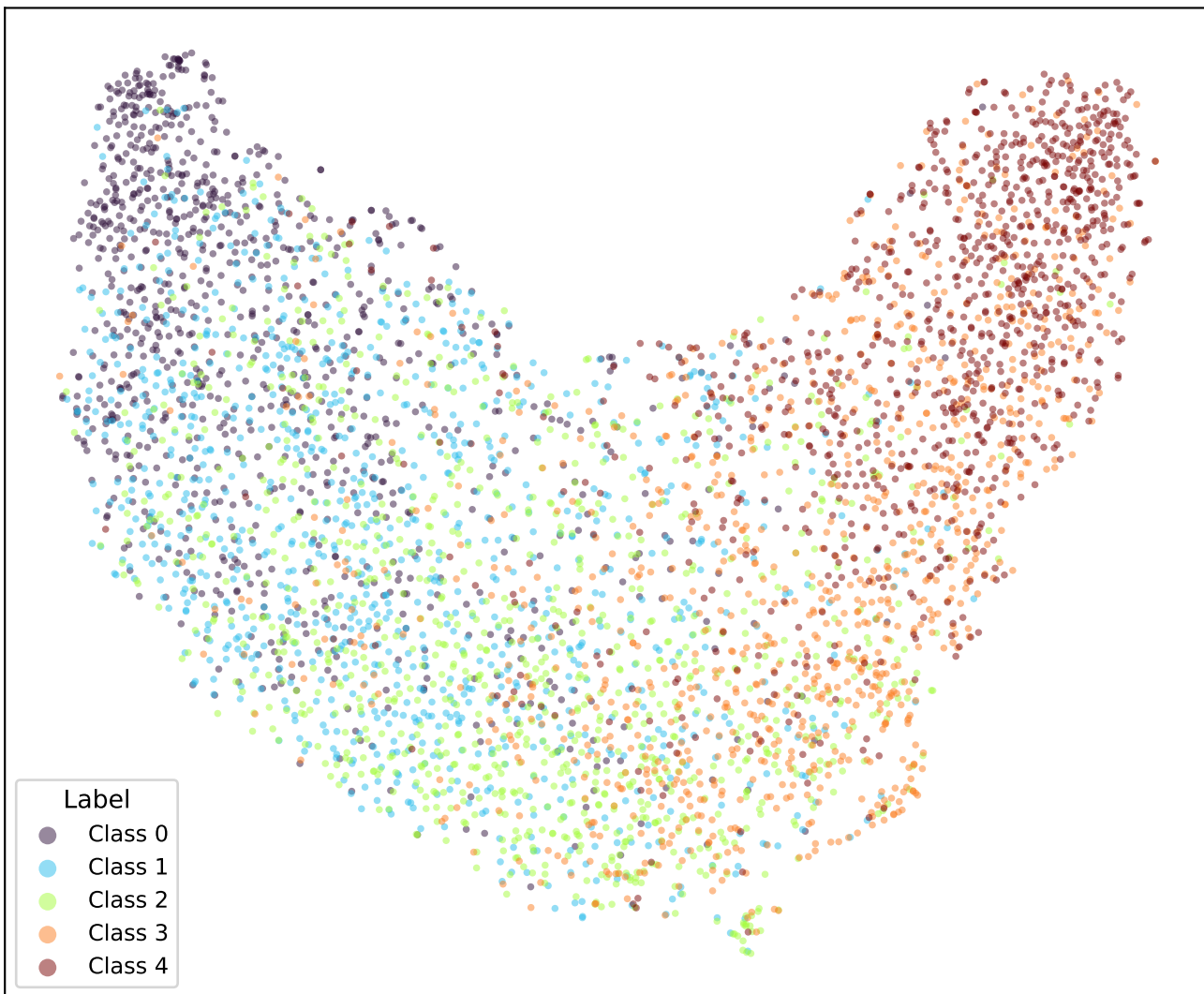
google/bert_uncased_L-2_H-128_A-2-amazon_reviews-CE-TRIPa2-4 (val)
