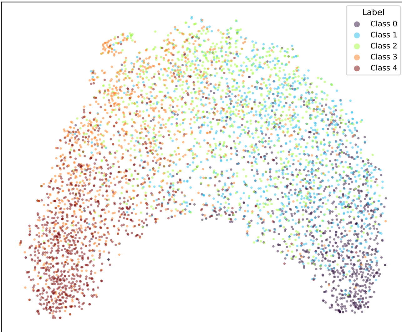
google/bert_uncased_L-2_H-128_A-2-amazon_reviews-CE-TRIPa2-5 (val)
