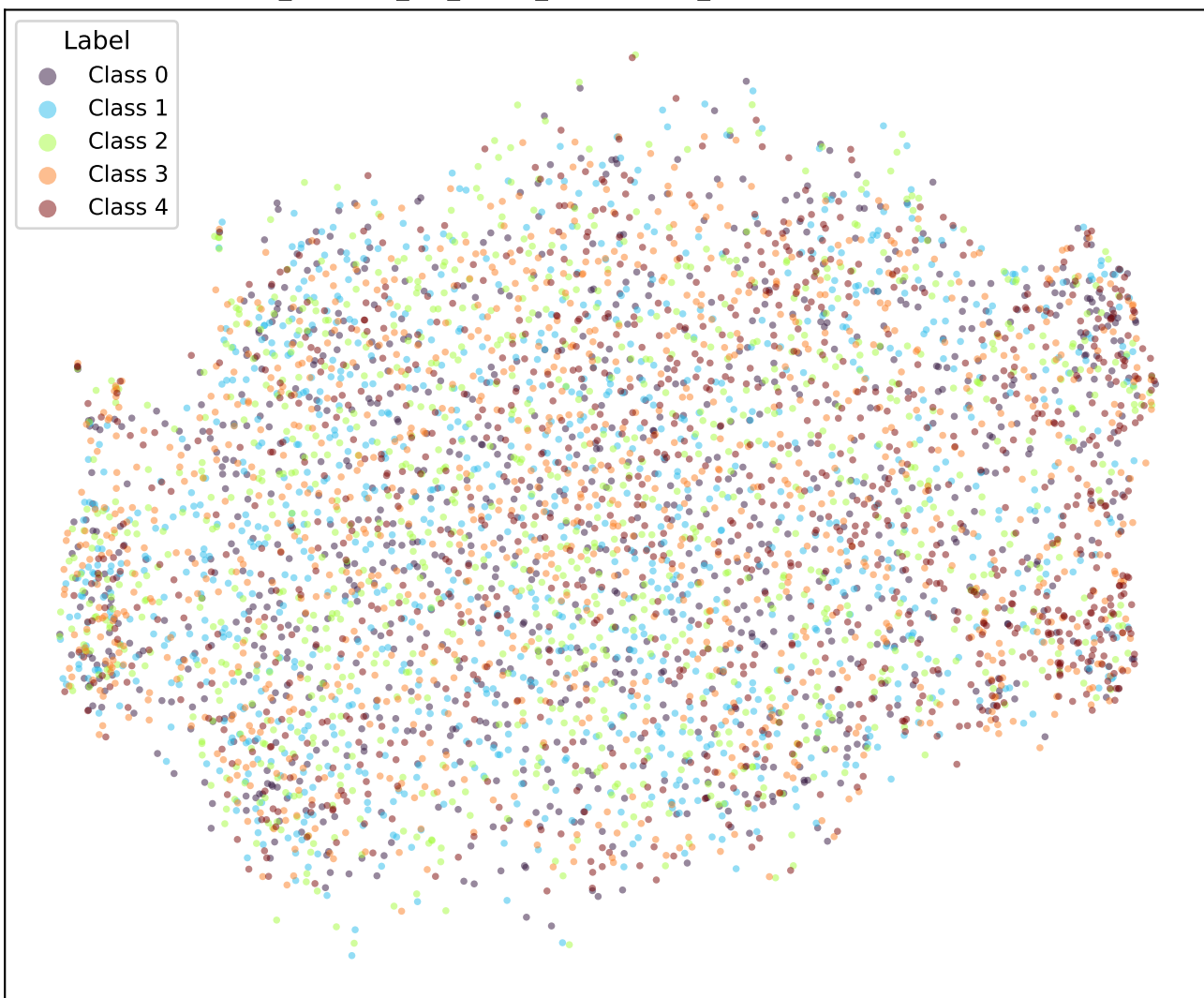
google/bert_uncased_L-2_H-128_A-2-amazon_reviews-CORAL-TRIPa2-2 (val)
