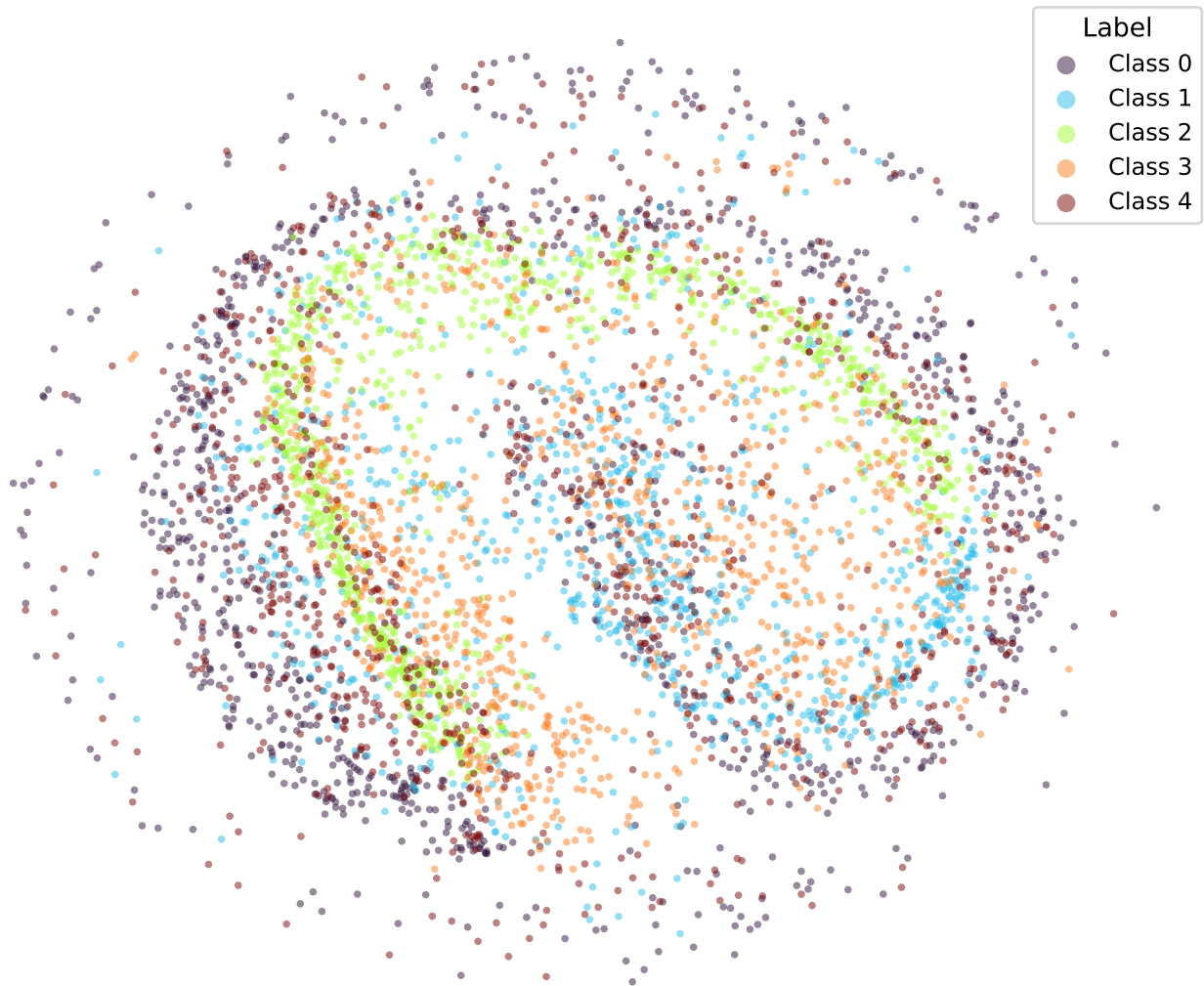
google/bert_uncased_L-2_H-128_A-2-amazon_reviews-CORAL-TRIPa2-3 (val)
