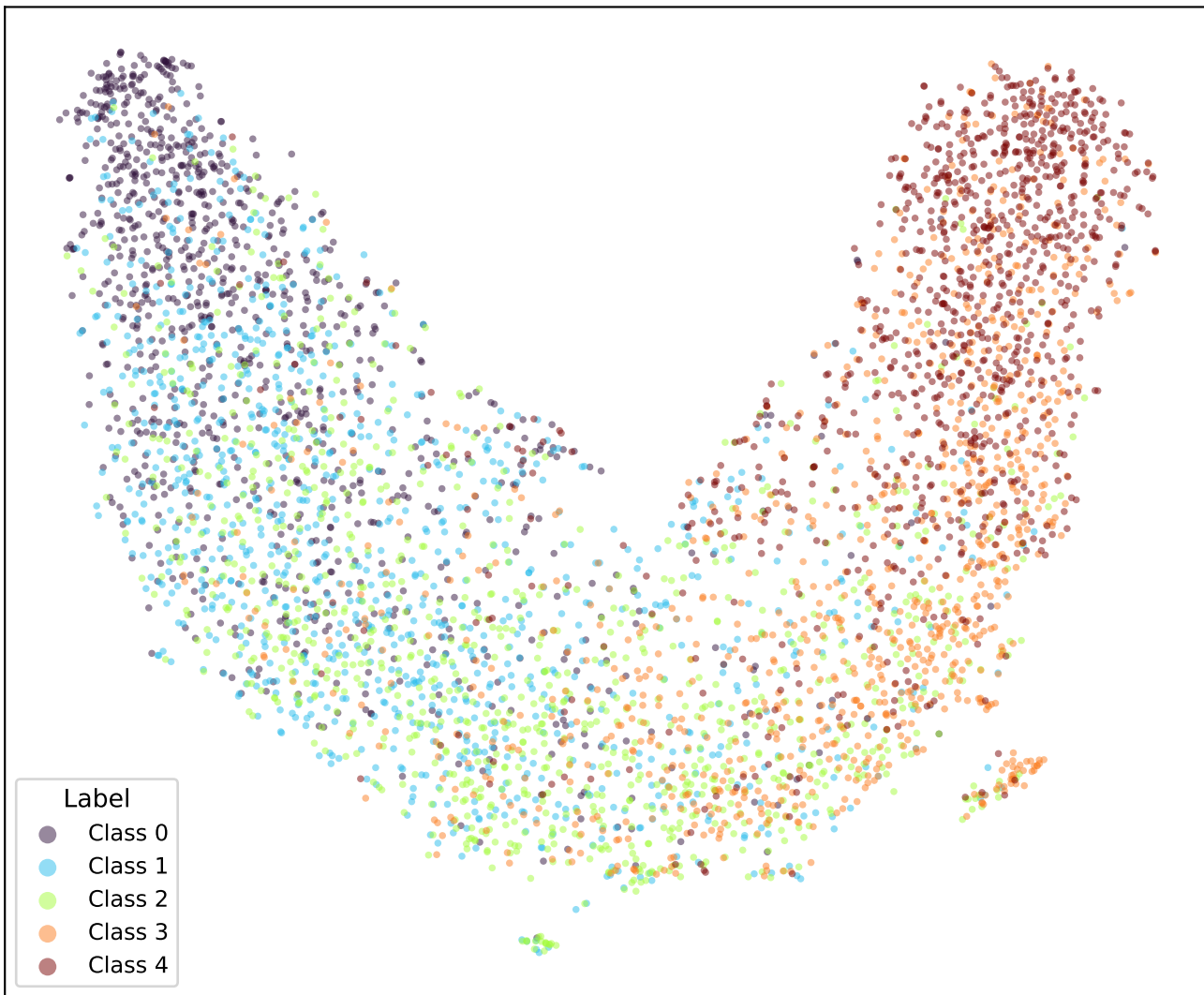
google/bert_uncased_L-2_H-128_A-2-amazon_reviews-EMD-TRIPa2-3 (val)
