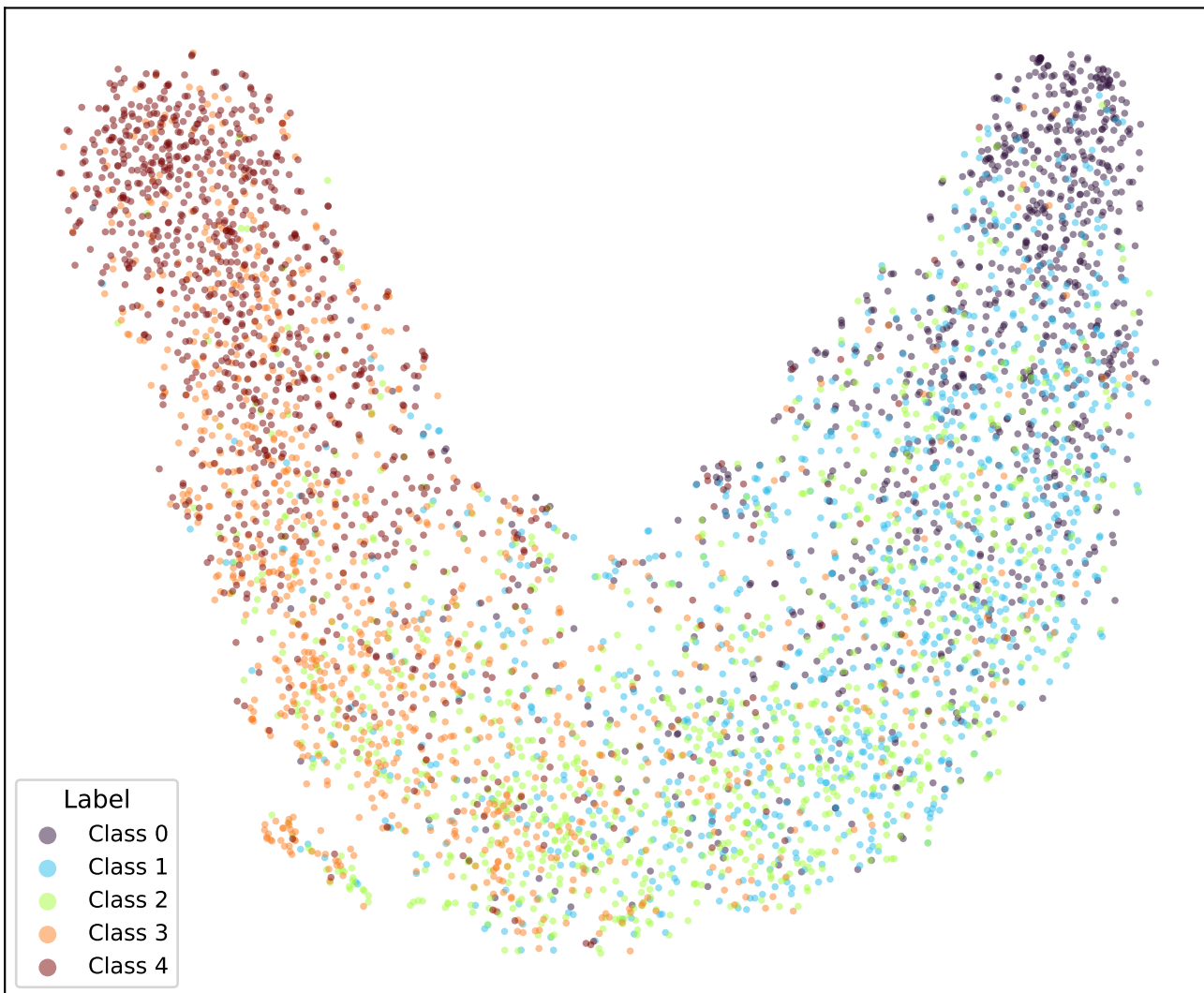
google/bert_uncased_L-2_H-128_A-2-amazon_reviews-EMD-TRIPa2-5 (val)
