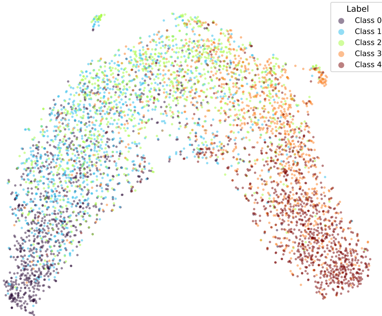
google/bert_uncased_L-2_H-128_A-2-amazon_reviews-OLL1-TRIPa2-1 (val)
