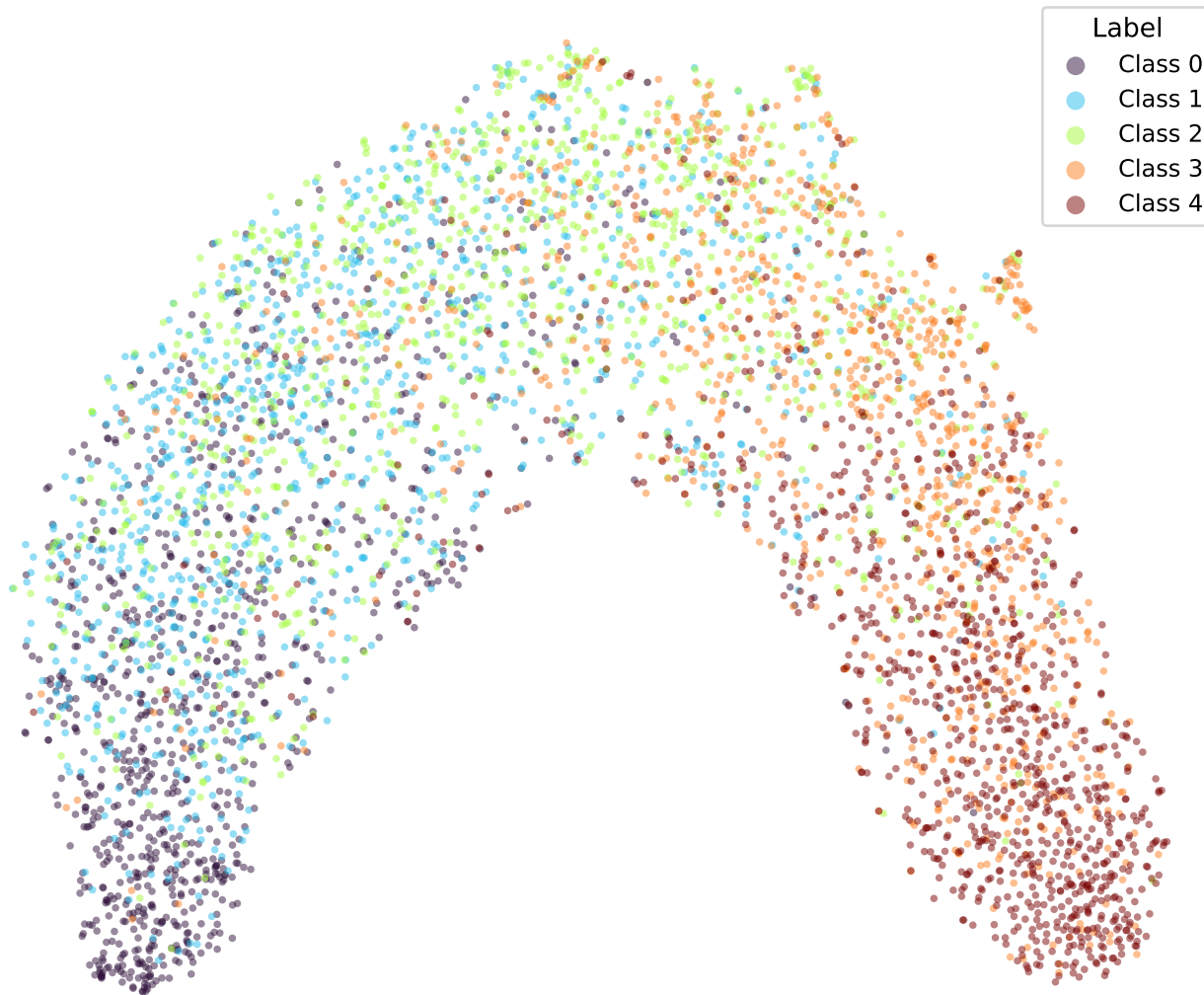
google/bert_uncased_L-2_H-128_A-2-amazon_reviews-OLL1-TRIPa2-2 (val)
