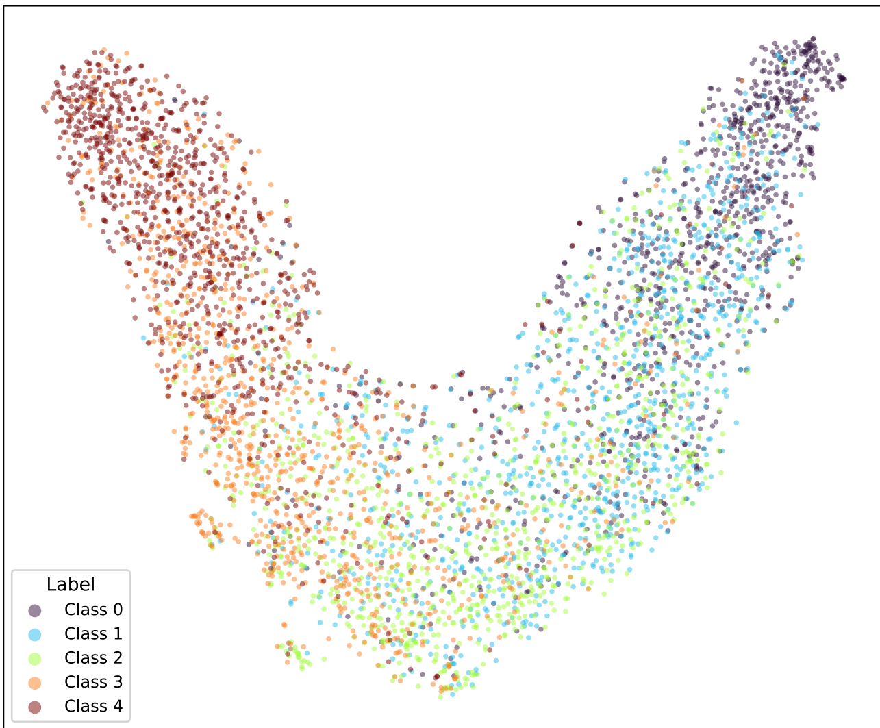
google/bert_uncased_L-2_H-128_A-2-amazon_reviews-OLL15-TRIPa2-4 (val)
