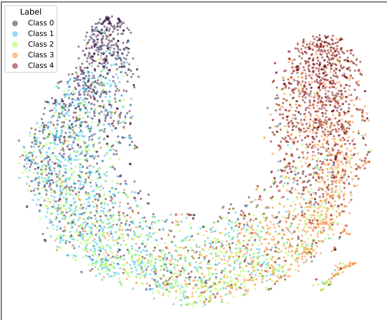
google/bert_uncased_L-2_H-128_A-2-amazon_reviews-OLL2-TRIPa2-5 (val)
