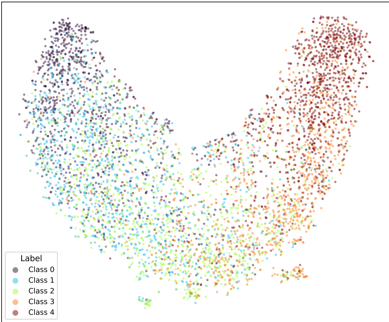
google/bert_uncased_L-2_H-128_A-2-amazon_reviews-SOFT2-TRIPa2-2 (val)
