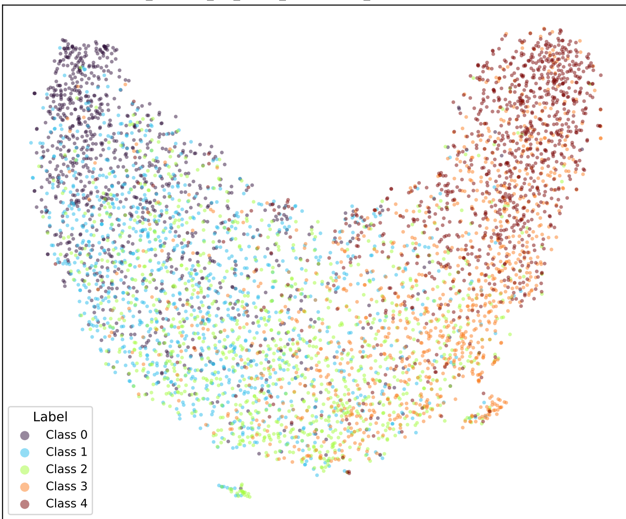
google/bert_uncased_L-2_H-128_A-2-amazon_reviews-SOFT2-TRIPa2-3 (val)
