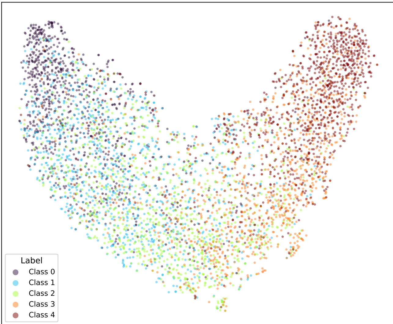
google/bert_uncased_L-2_H-128_A-2-amazon_reviews-SOFT2-TRIPa2-4 (val)
