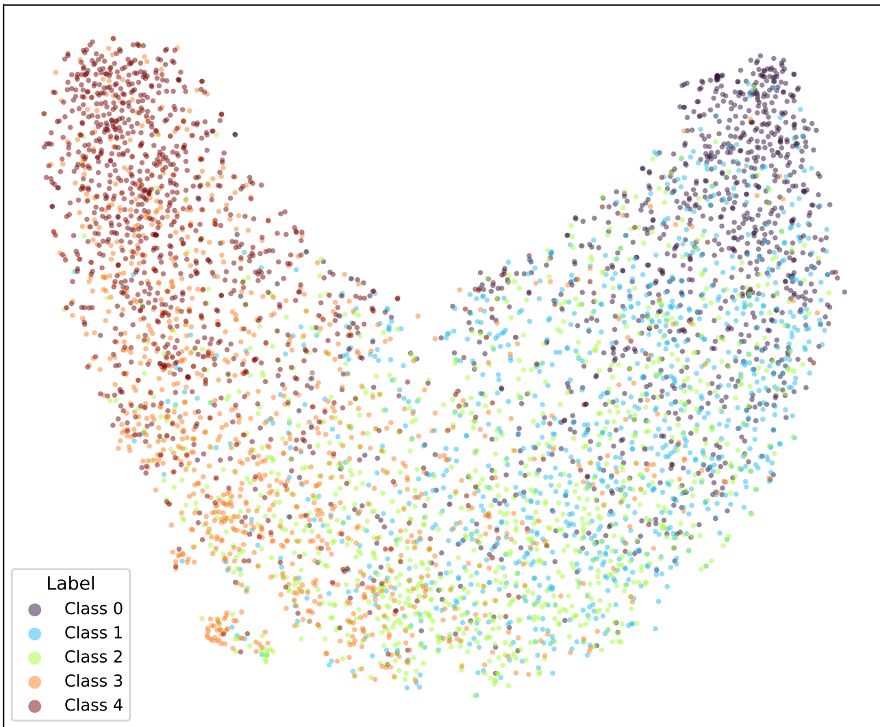
google/bert_uncased_L-2_H-128_A-2-amazon_reviews-SOFT2-TRIPa2-5 (val)
