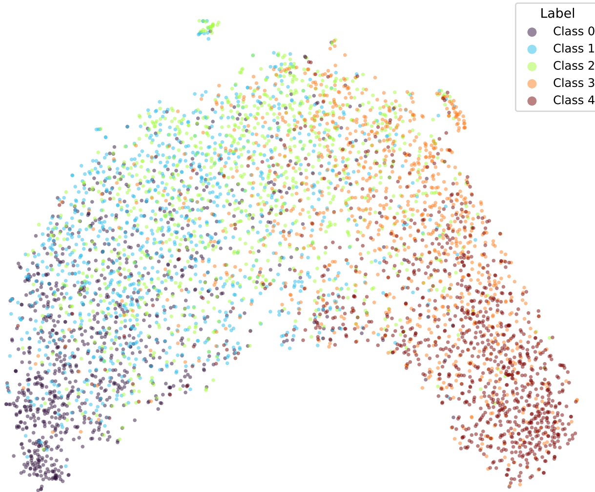
google/bert_uncased_L-2_H-128_A-2-amazon_reviews-SOFT3-TRIPa2-1 (val)
