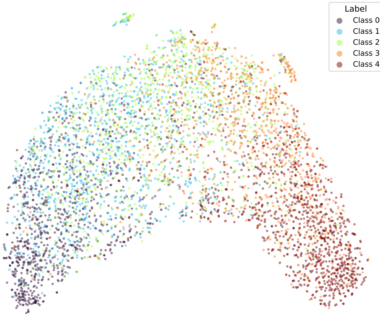
google/bert_uncased_L-2_H-128_A-2-amazon_reviews-SOFT4-TRIPa2-1 (val)
