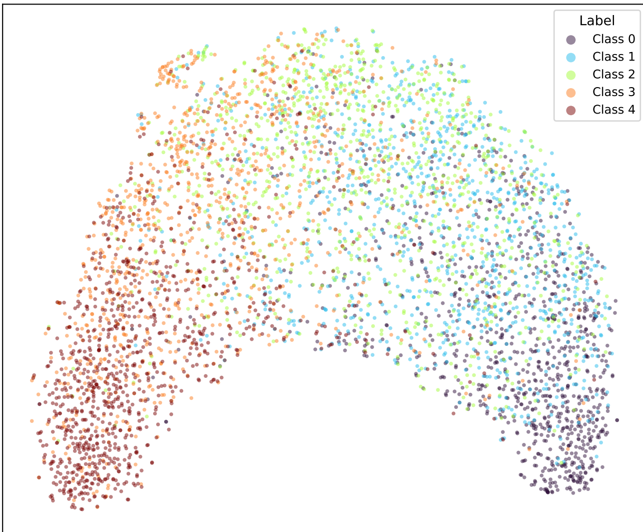
google/bert_uncased_L-2_H-128_A-2-amazon_reviews-SOFT4-TRIPa2-5 (val)
