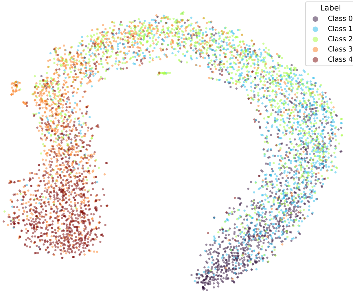
google/bert_uncased_L-2_H-128_A-2-amazon_reviews-WKL-TRIPa2-3 (val)
