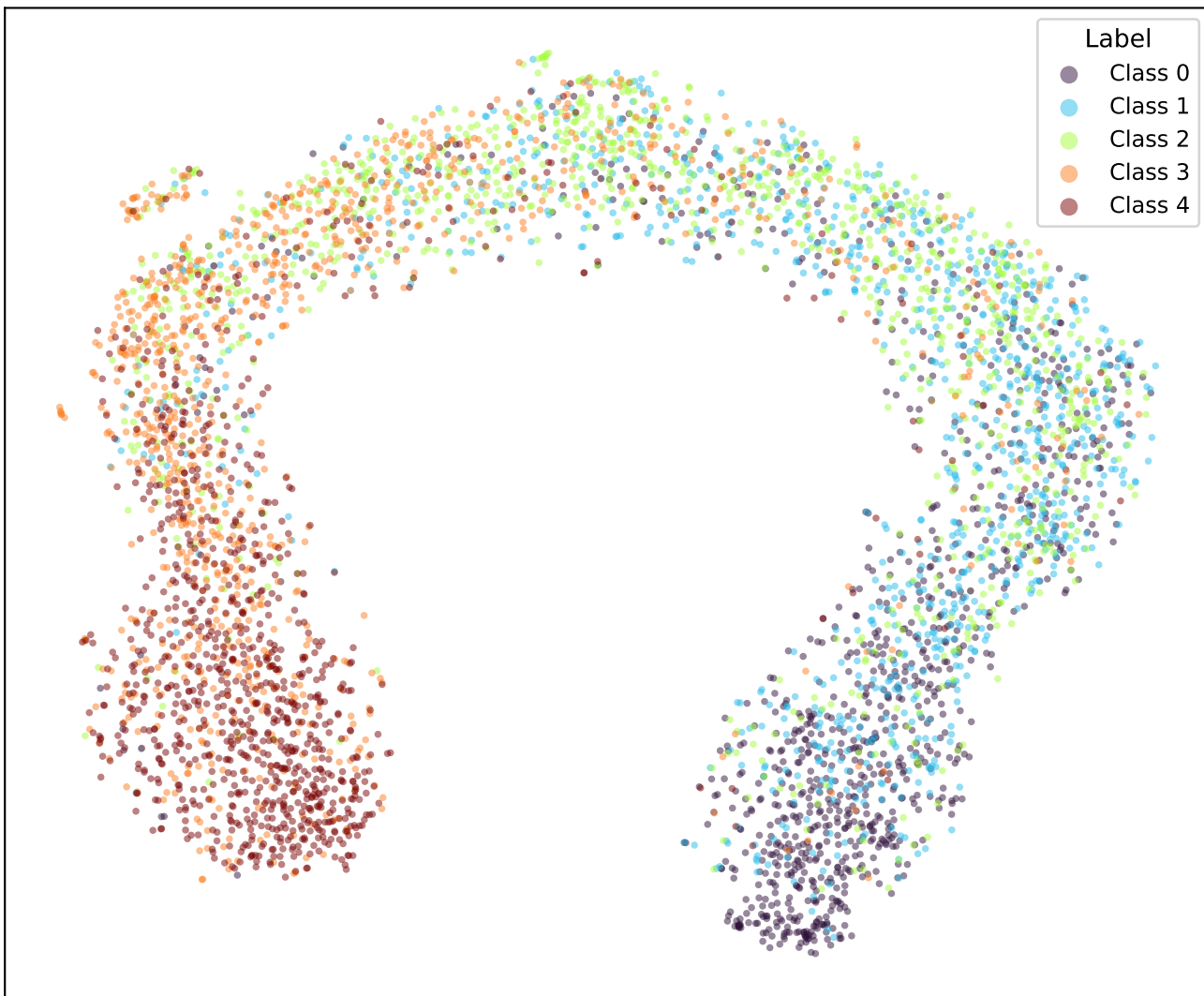
google/bert_uncased_L-2_H-128_A-2-amazon_reviews-WKL-TRIPa2-4 (val)
