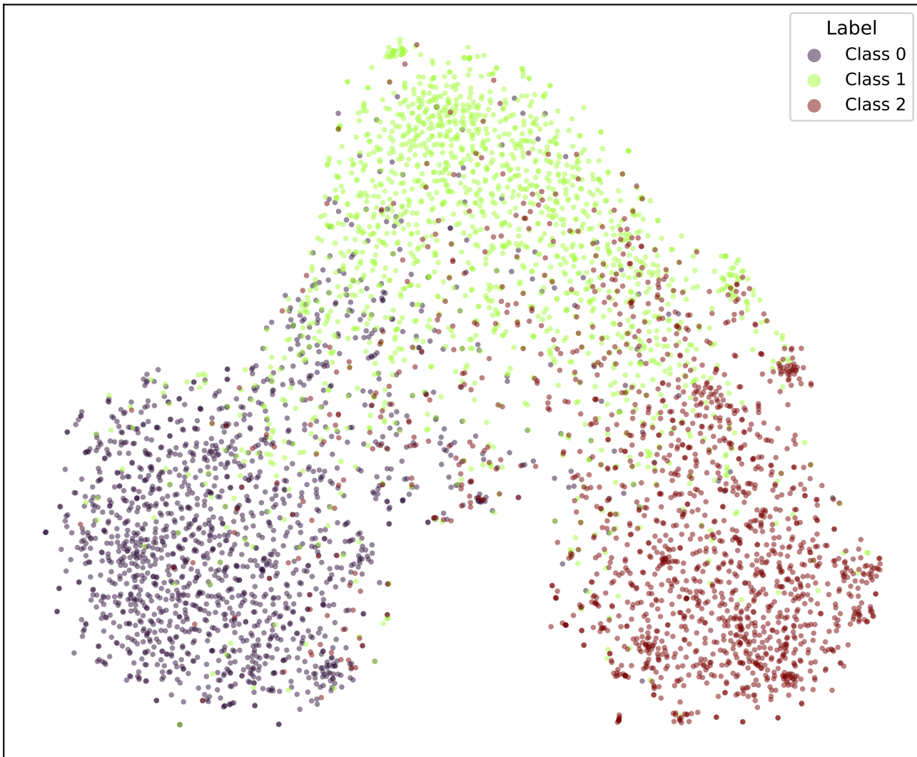
google/bert_uncased_L-2_H-128_A-2-snli-CE-TRIPa2-1 (val)
