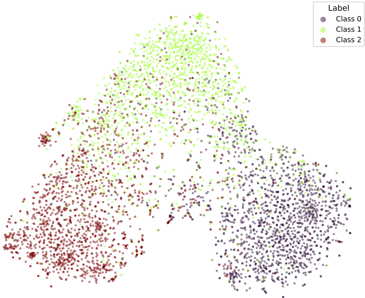
google/bert_uncased_L-2_H-128_A-2-snli-CE-TRIPa2-2 (val)
