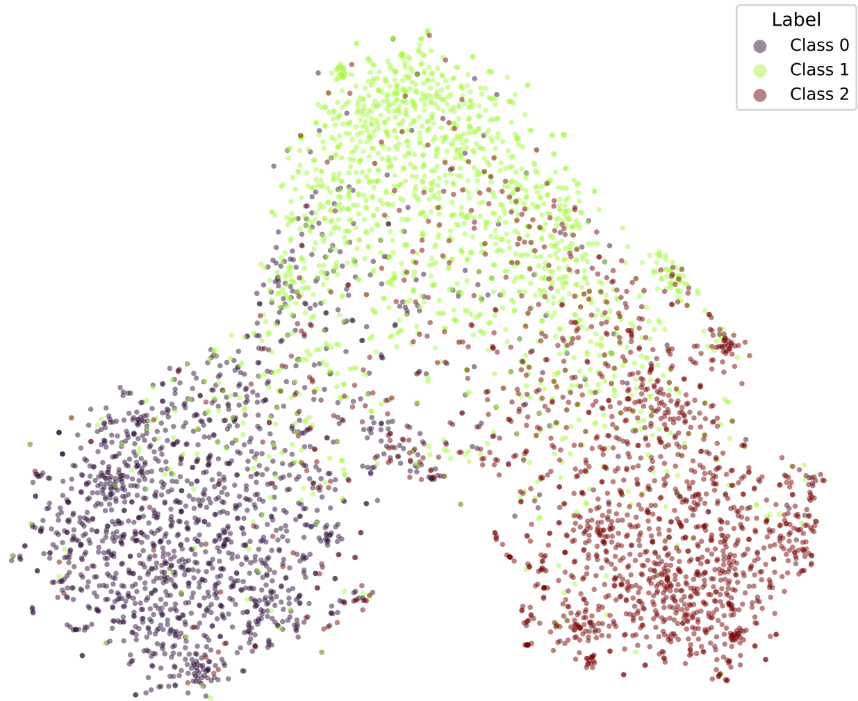
google/bert_uncased_L-2_H-128_A-2-snli-CE-TRIPa2-3 (val)
