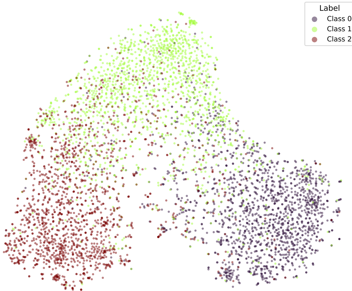
google/bert_uncased_L-2_H-128_A-2-snli-CE-TRIPa2-4 (val)
