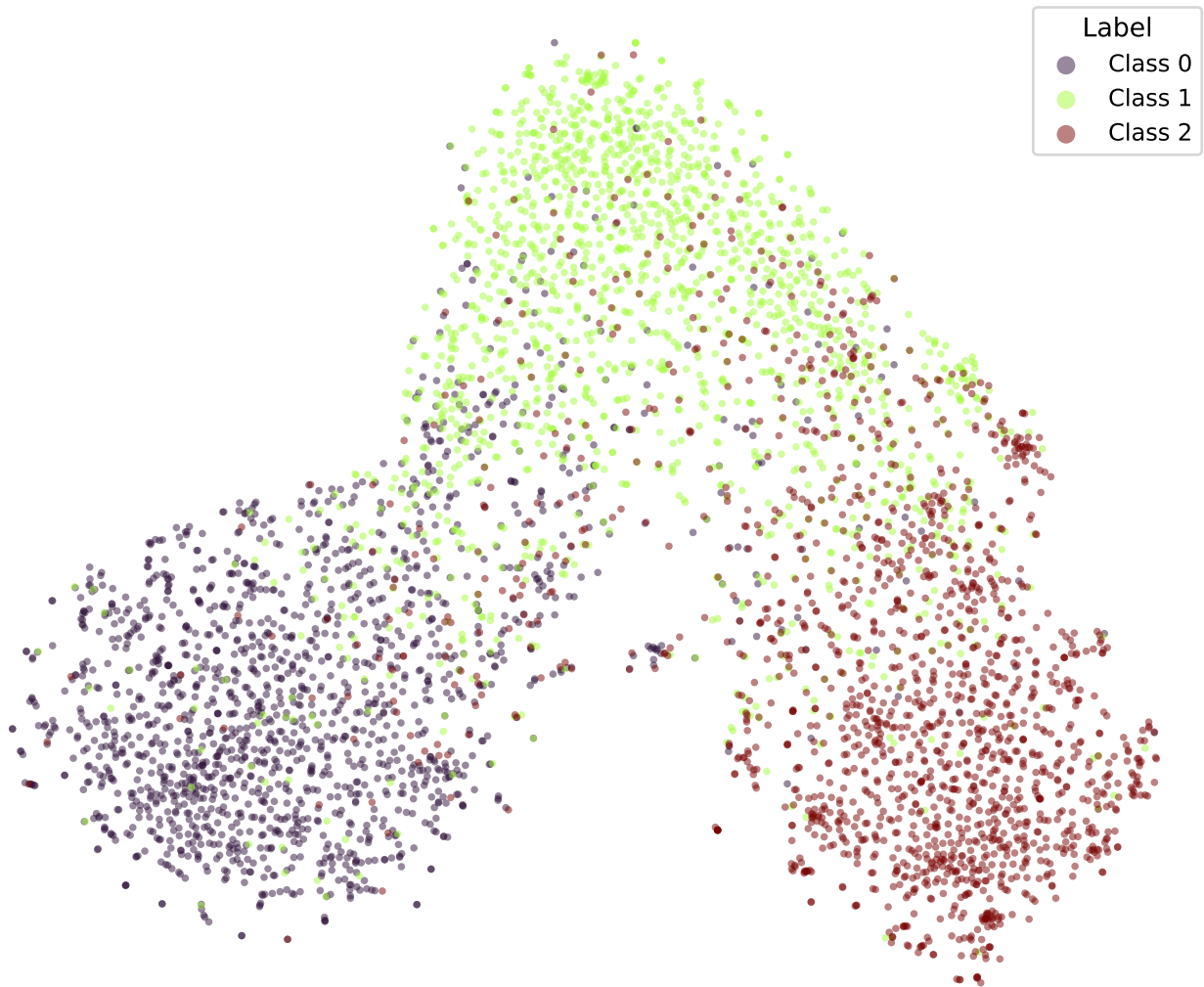
google/bert_uncased_L-2_H-128_A-2-snli-OLL1-TRIPa2-3 (val)
