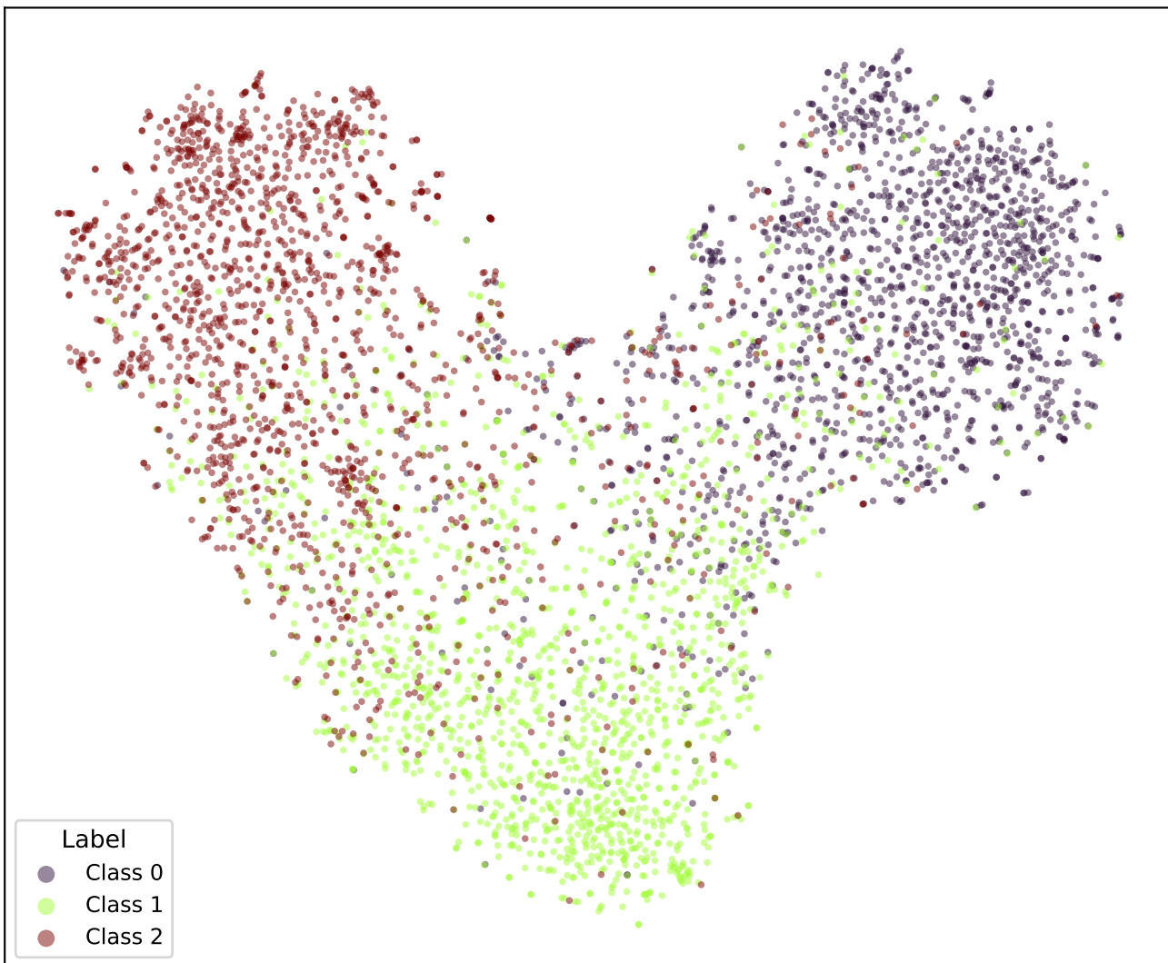
google/bert_uncased_L-2_H-128_A-2-snli-OLL15-TRIPa2-4 (val)
