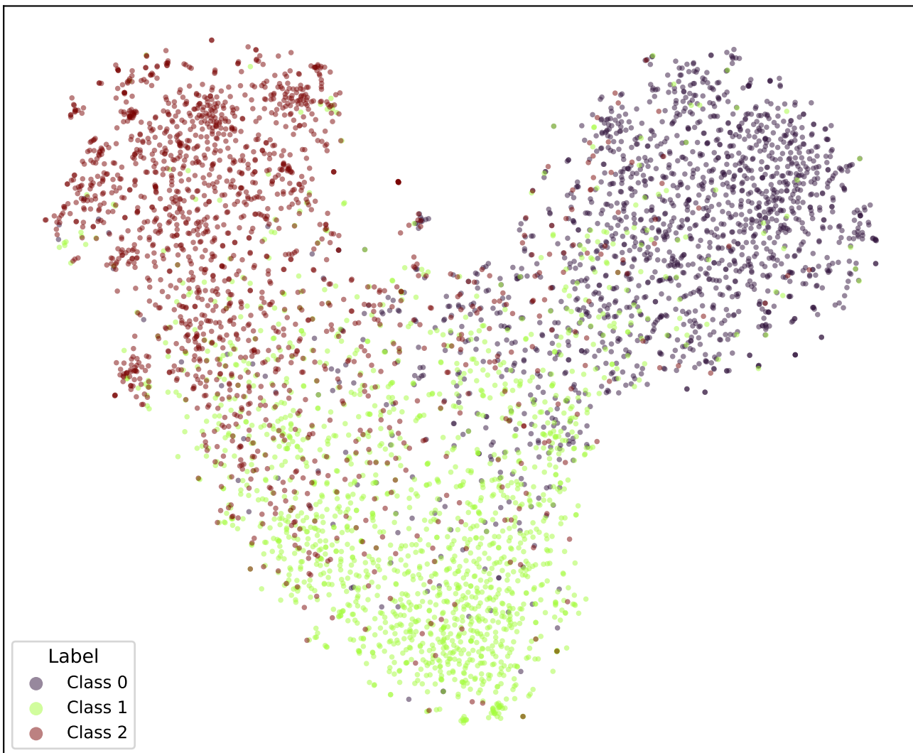
google/bert_uncased_L-2_H-128_A-2-snli-OLL15-TRIPa2-5 (val)
