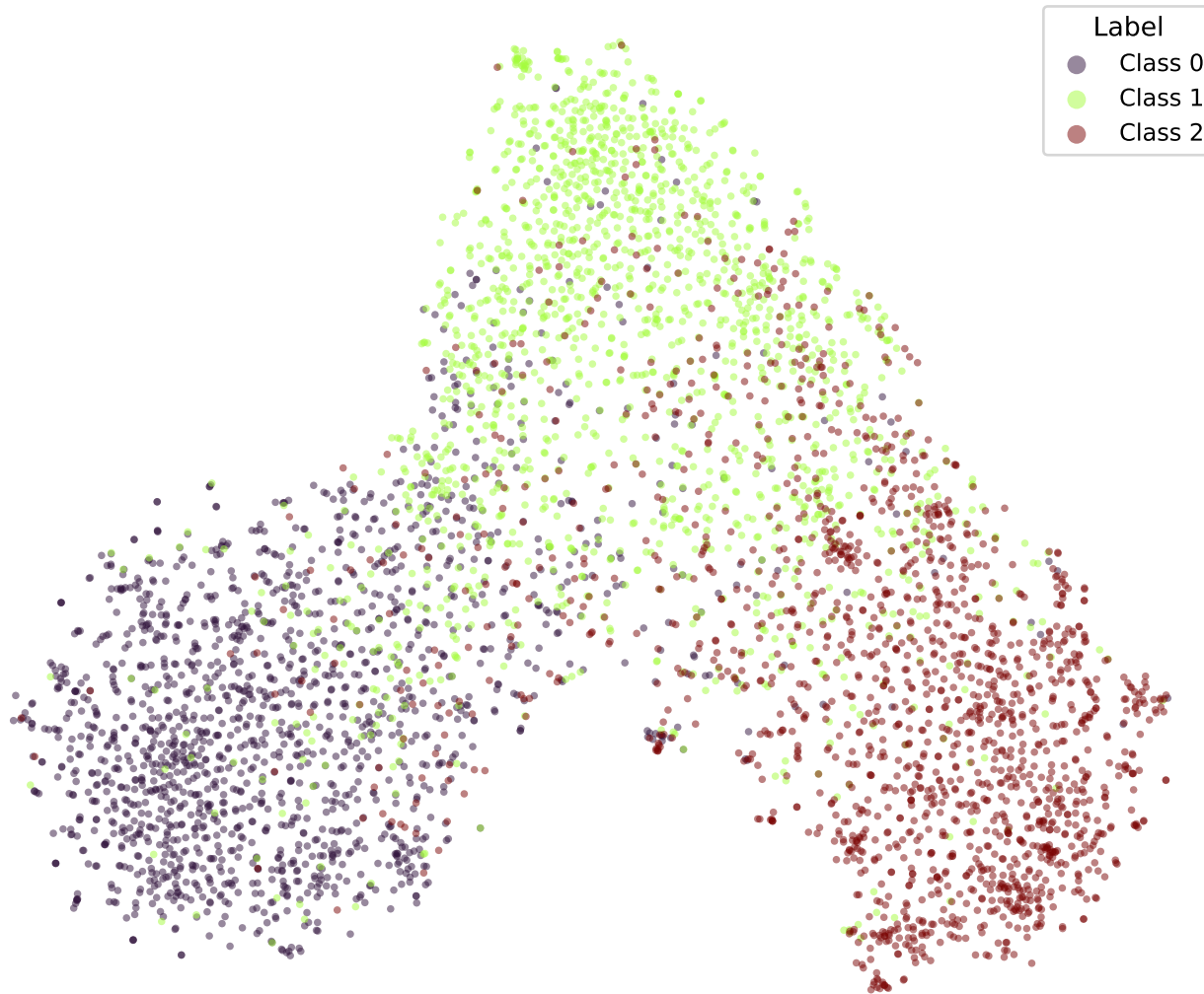
google/bert_uncased_L-2_H-128_A-2-snli-OLL2-TRIPa2-2 (val)
