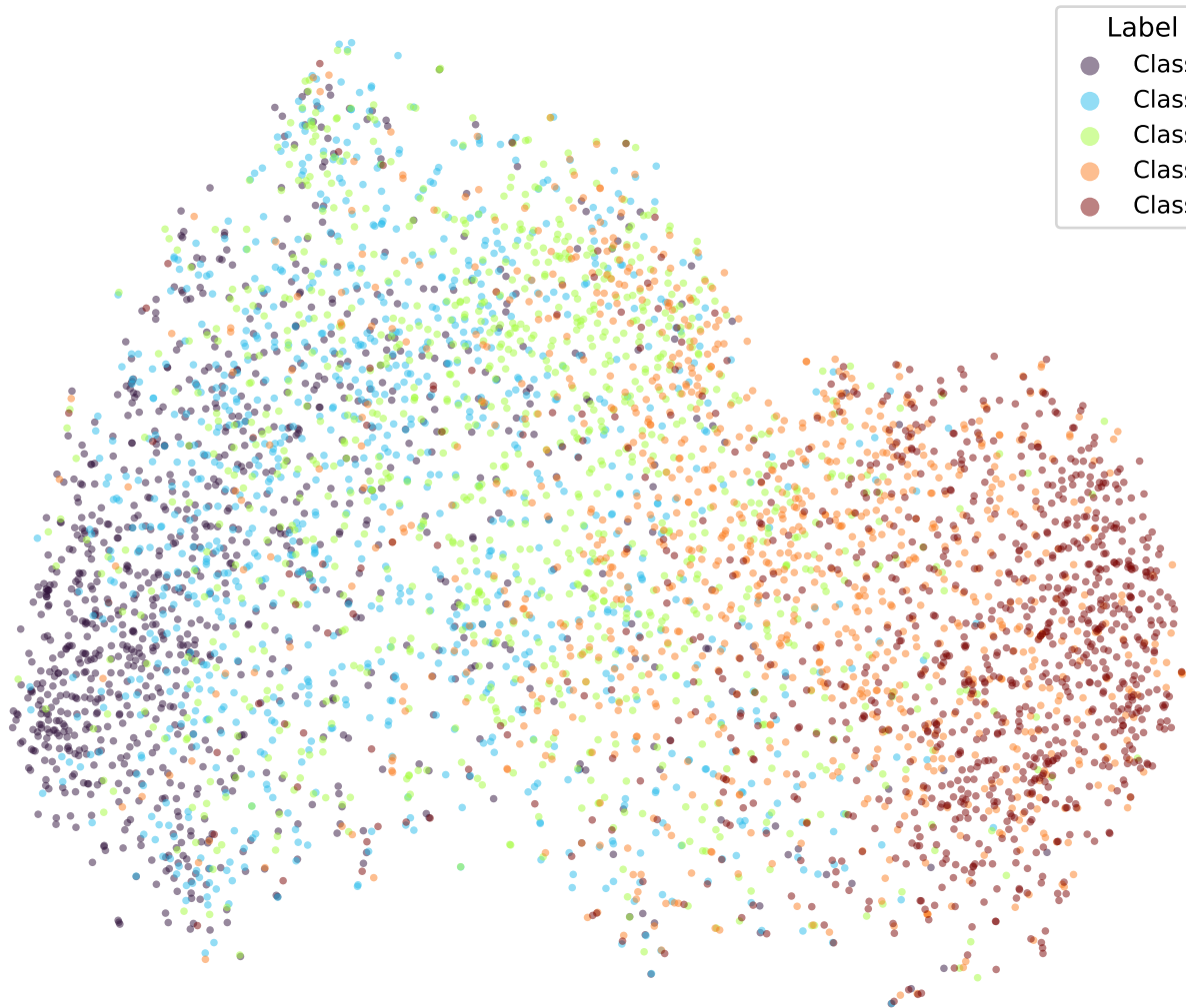
t-SNE | bert-tiny-amazon_reviews-k1-adaptive-cosine (epoch 7.0)
