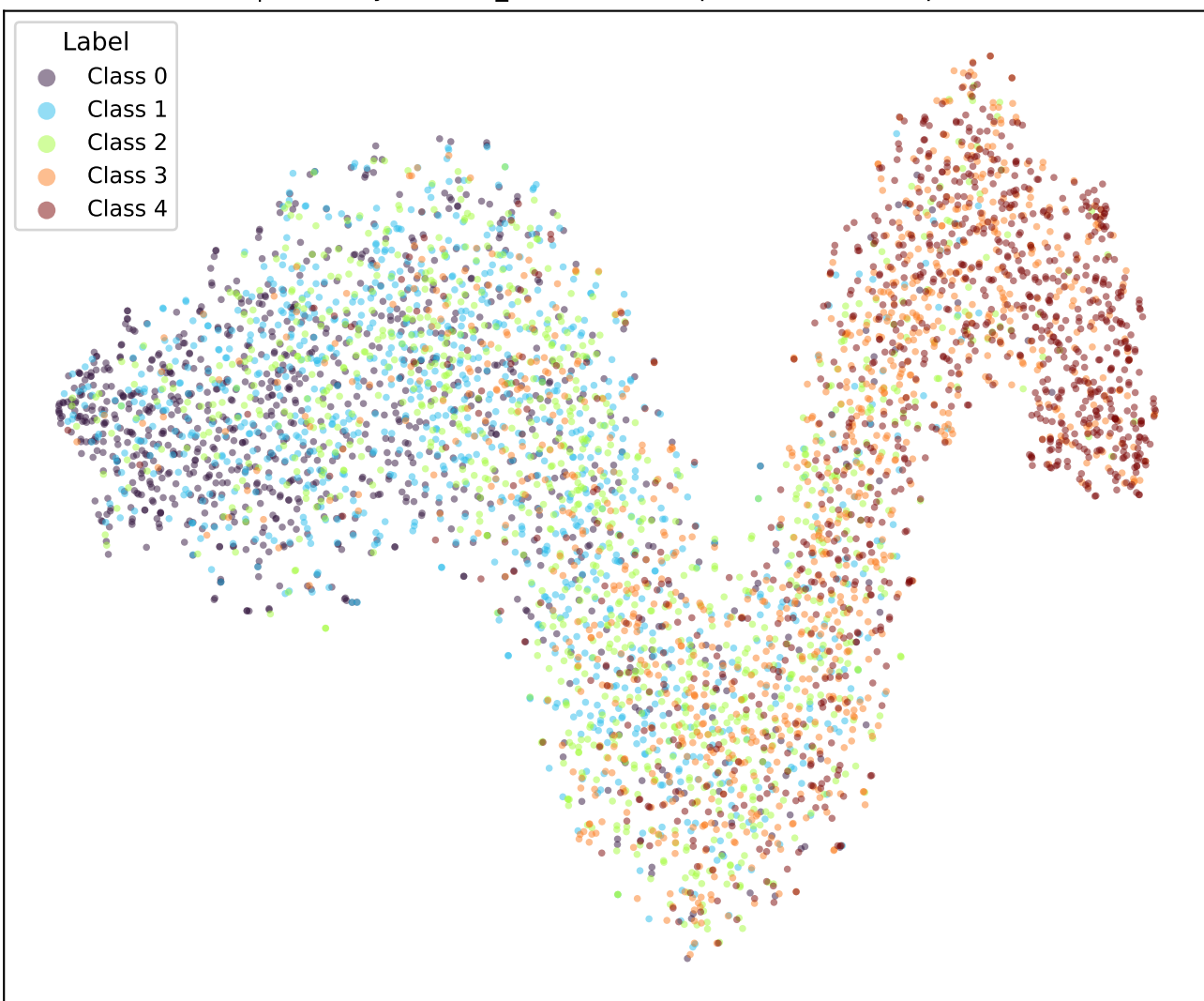
t-SNE | bert-tiny-amazon_reviews-k1-adaptive-euclidean (epoch 1.0)
