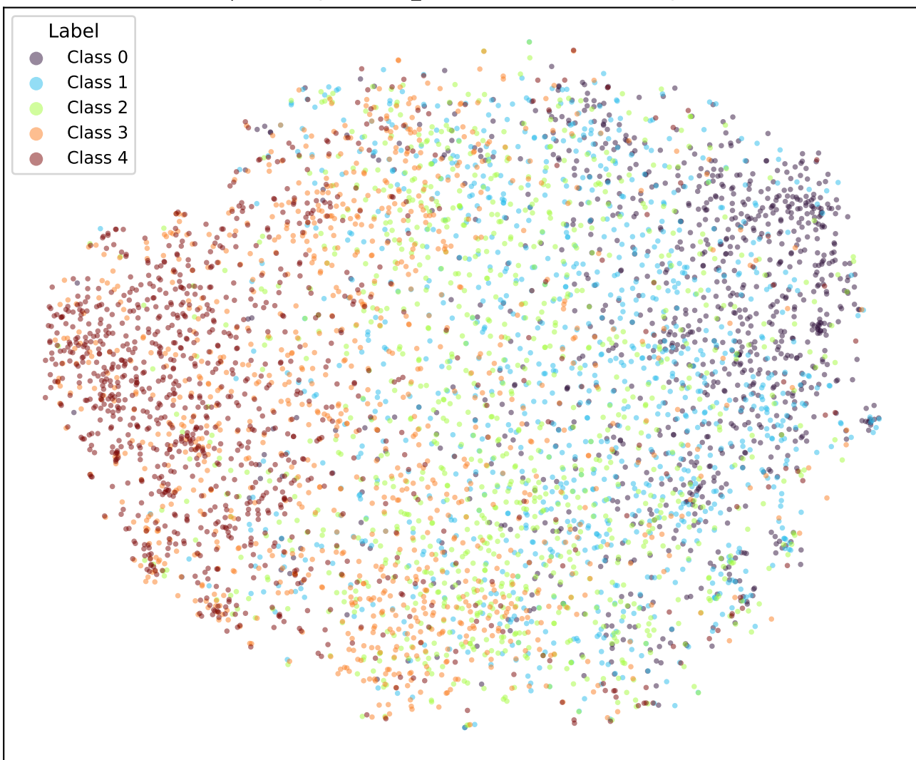
t-SNE | bert-tiny-amazon_reviews-k1-fixed-cosine (epoch 3.0)
