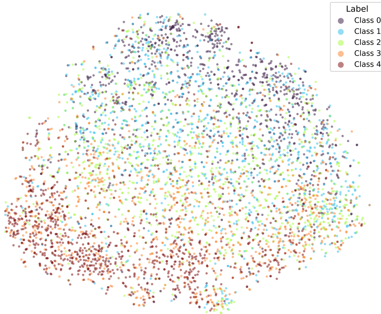
t-SNE | bert-tiny-amazon_reviews-k3-fixed-cosine (epoch 1.0)
