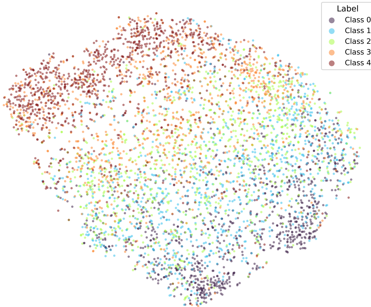
t-SNE | bert-tiny-amazon_reviews-k3-fixed-cosine (epoch 5.0)
