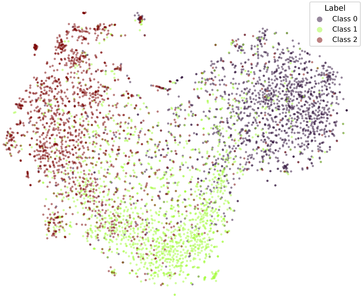
t-SNE | bert-tiny-snli-k1-adaptive-cosine
