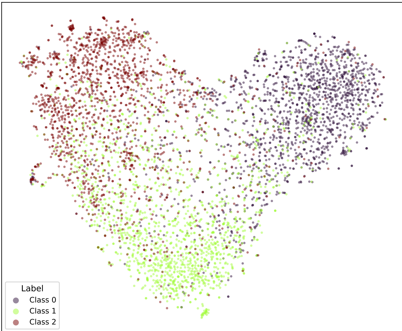
t-SNE | bert-tiny-snli-k1-fixed-cosine
