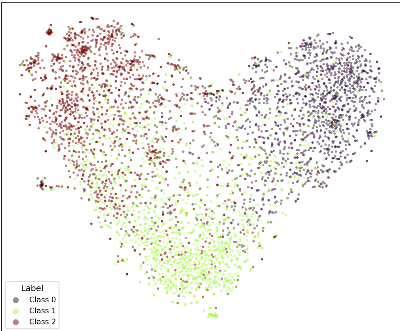
t-SNE | bert-tiny-snli-k1-fixed-cosine (epoch 5.0)
