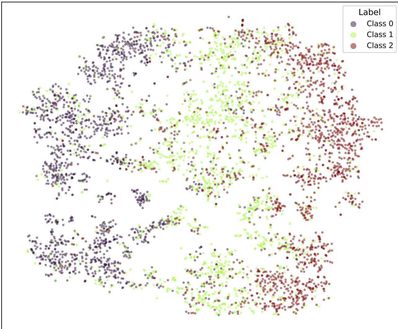
t-SNE | bert-tiny-snli-k10-adaptive-cosine (epoch 3.0)
