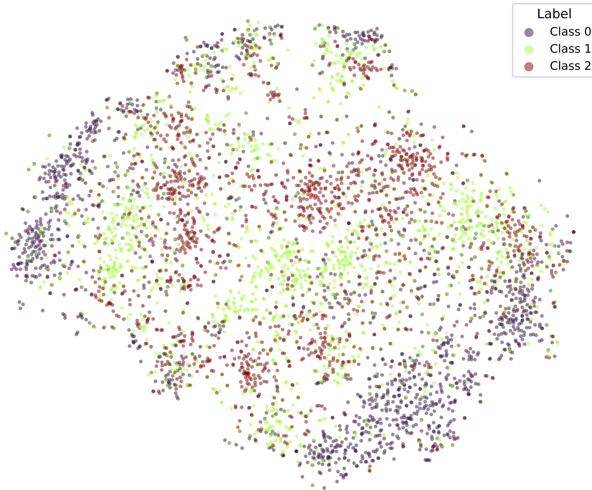
t-SNE | bert-tiny-snli-k10-fixed-cosine (epoch 1.0)
