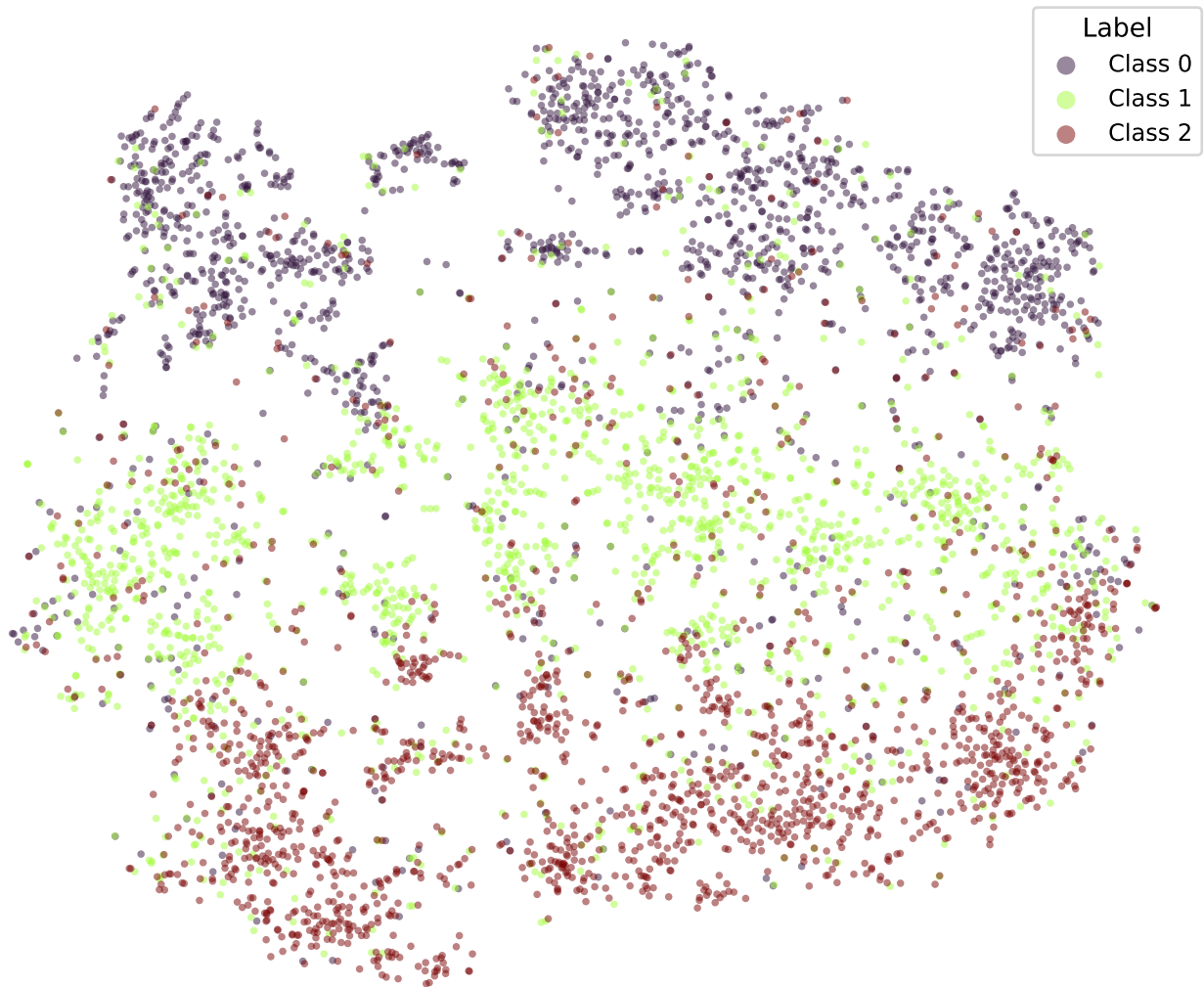
t-SNE | bert-tiny-snli-k10-fixed-cosine (epoch 3.0)
