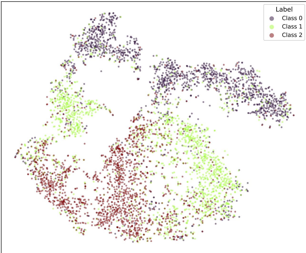
t-SNE | bert-tiny-snli-k3-fixed-cosine
