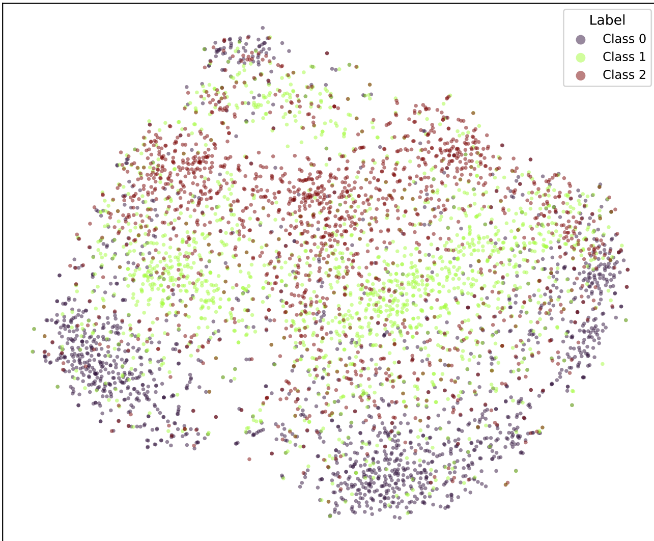
t-SNE | bert-tiny-snli-k3-fixed-cosine (epoch 1.0)
