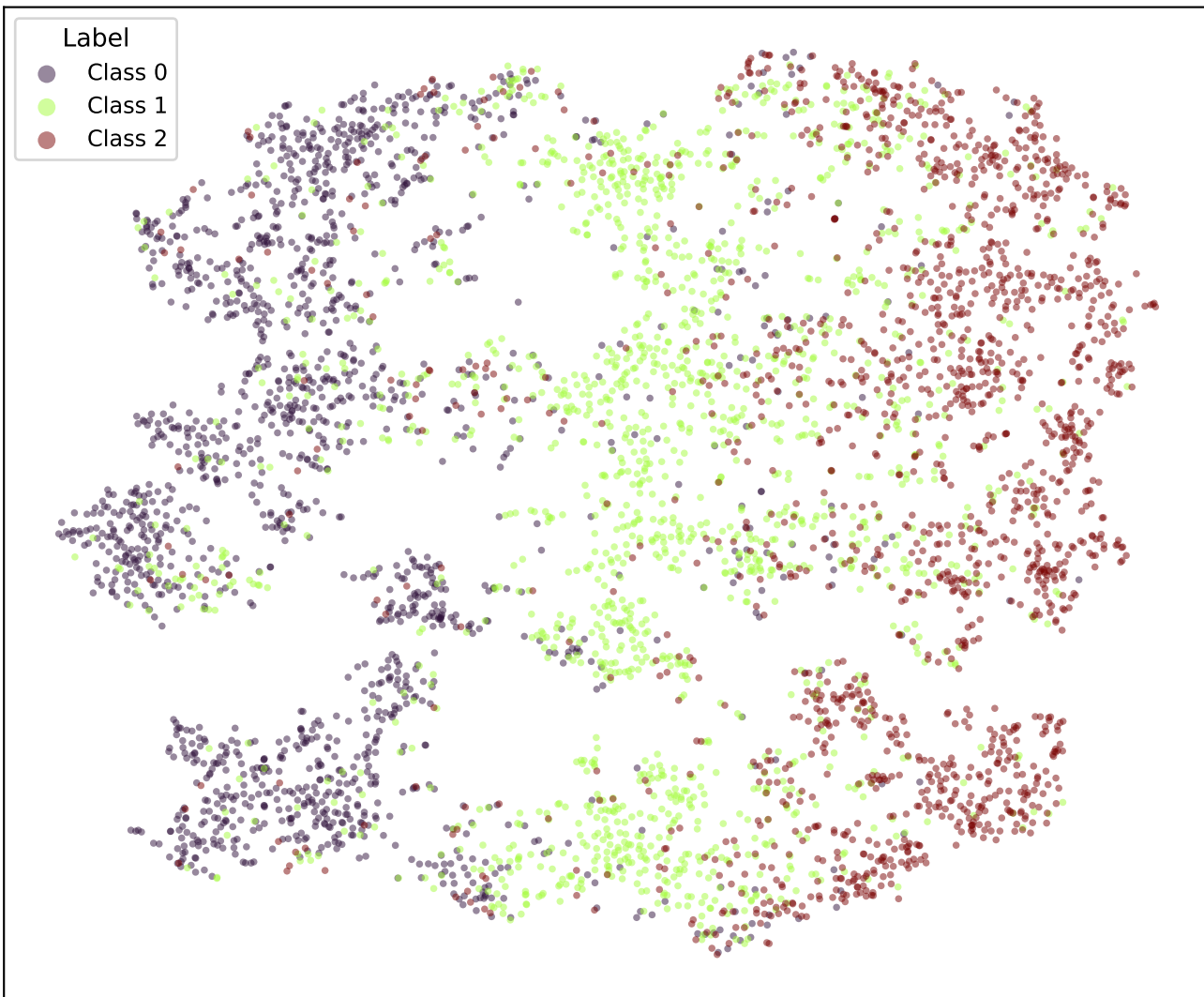
t-SNE | bert-tiny-snli-k5-adaptive-cosine
