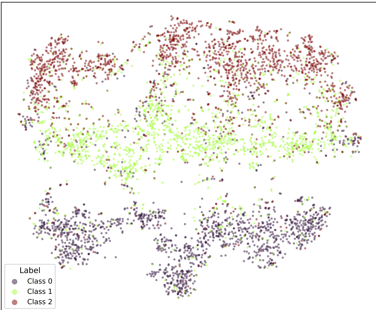
t-SNE | bert-tiny-snli-k5-fixed-cosine
